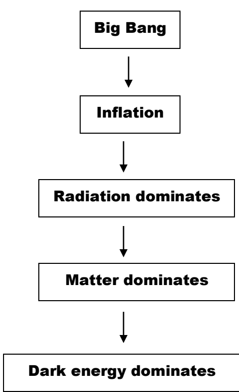
Inflationary model
