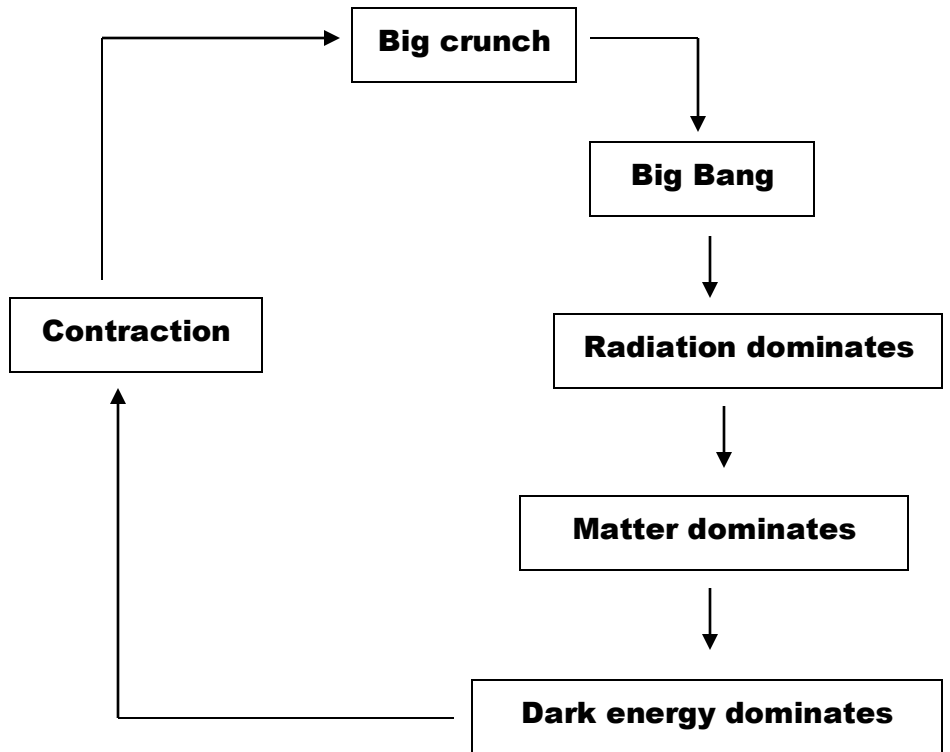
Cyclic model
